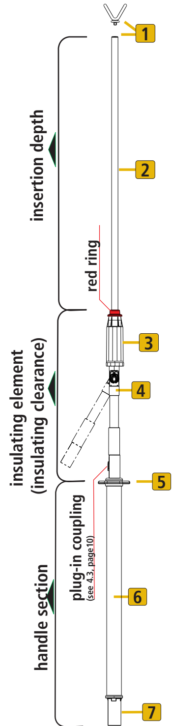
Insulating stick, IT ZK30 STK 30 360 (with gear coupling)
