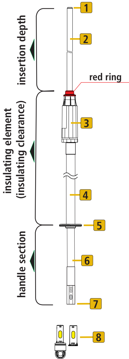
Insulating stick, IS M12 STK 640 (with M12 thread)
