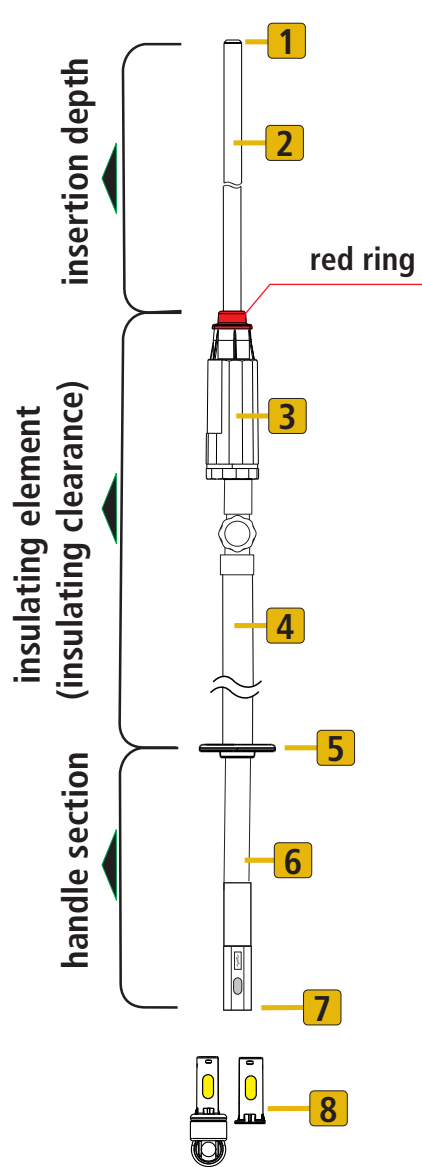
Insulating stick, IS ZK STK 670 (with gear coupling)
